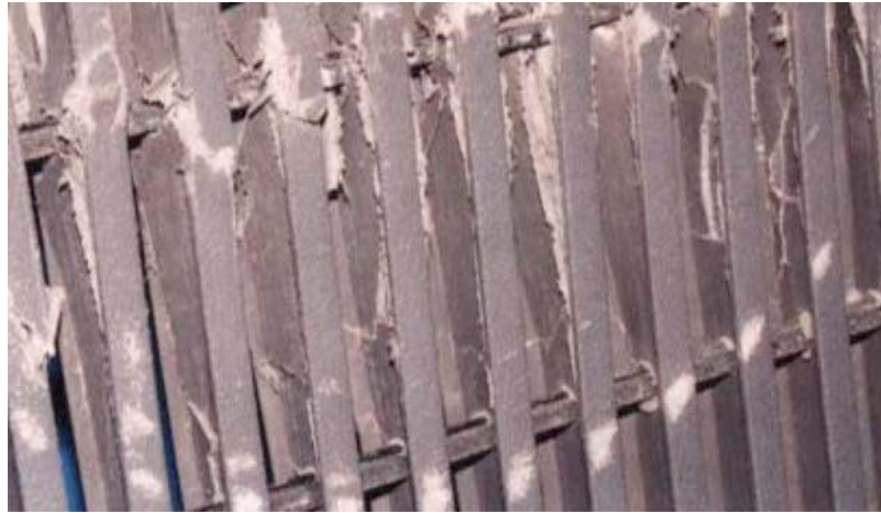
FIG. X2.2 Extensive Damage to Bearing Bars
